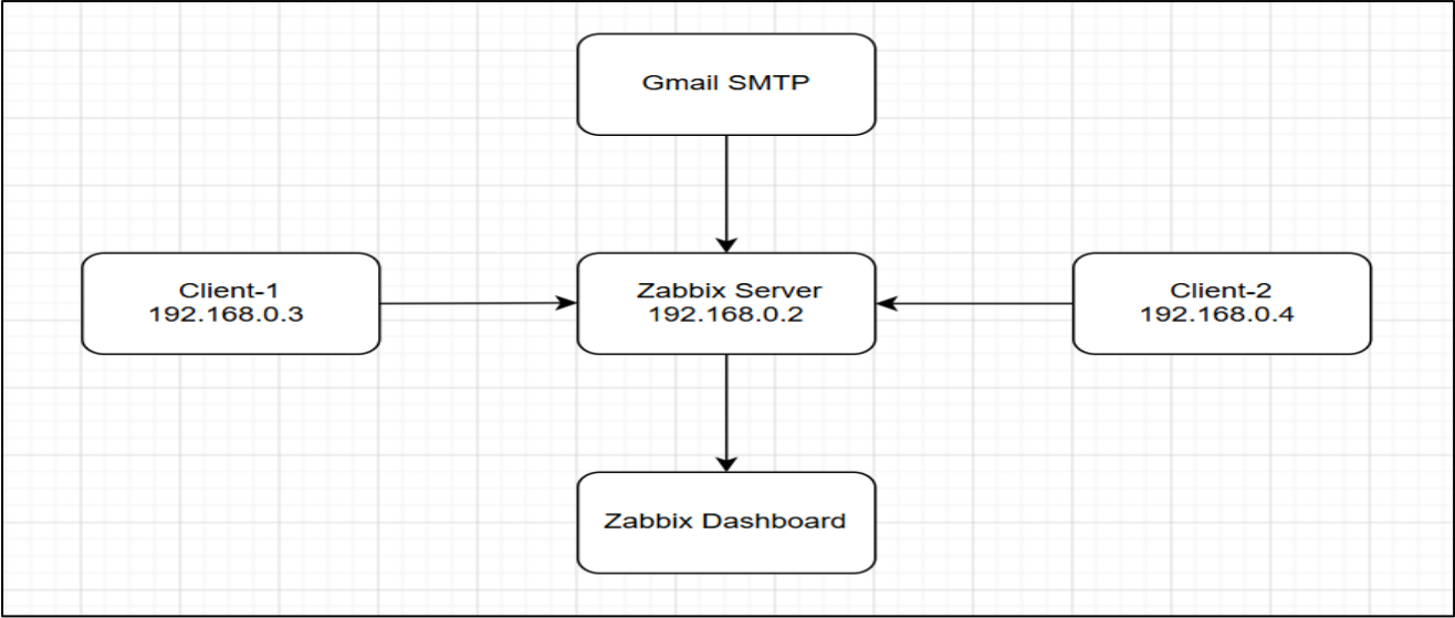
Figure: Project Architecture
