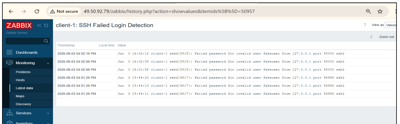
Figure: SSH Failed Login Monitoring
