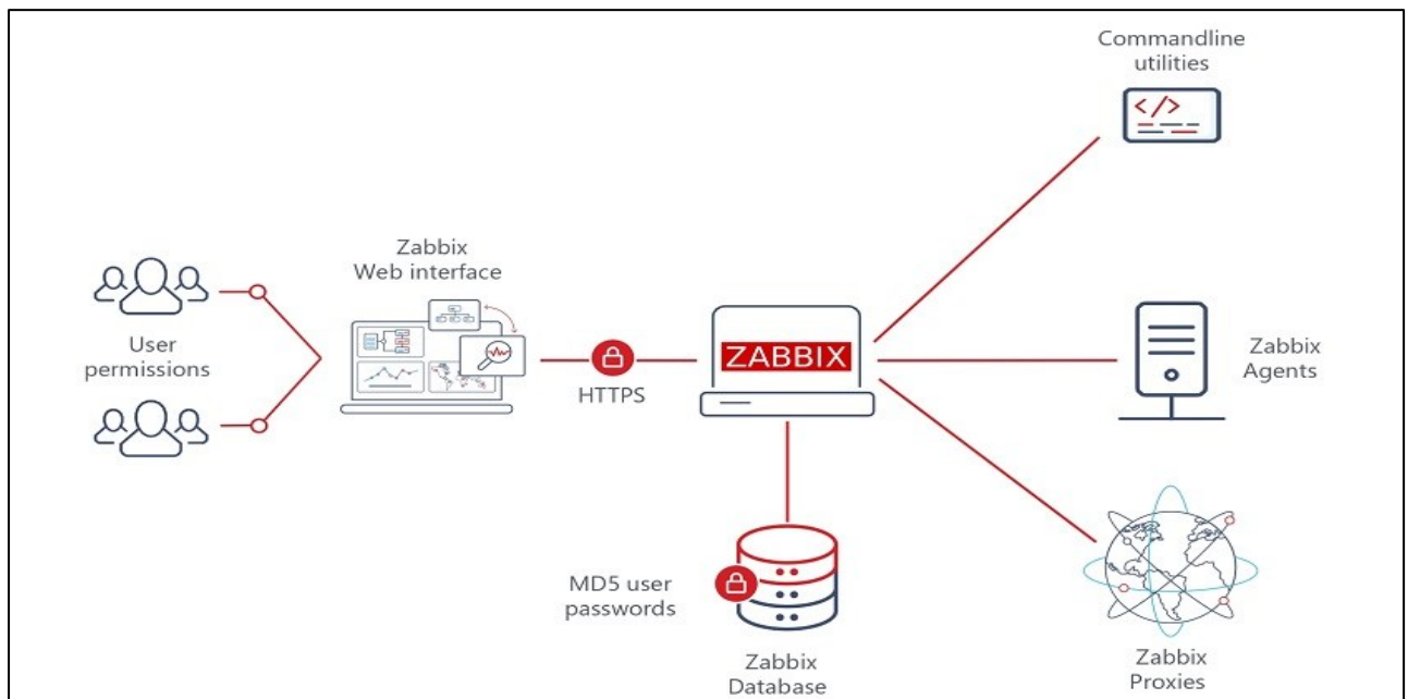
Figure: Architecture of Zabbix
